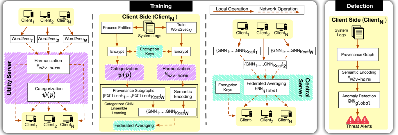
Fig. 2: High-level architecture of MIRAGE. In the training phase, our system builds local provenance graphs for each client and trains an ensemble of GNN models. Prior to this, we harmonize Word2vec models in a privacy preserving manner using encryption and dual-server architecture for semantic encoding. The local GNN models participate in federated learning to develop a global GNN_{global} model, which is then utilized for anomaly detection. Notations are defined in Table I.
