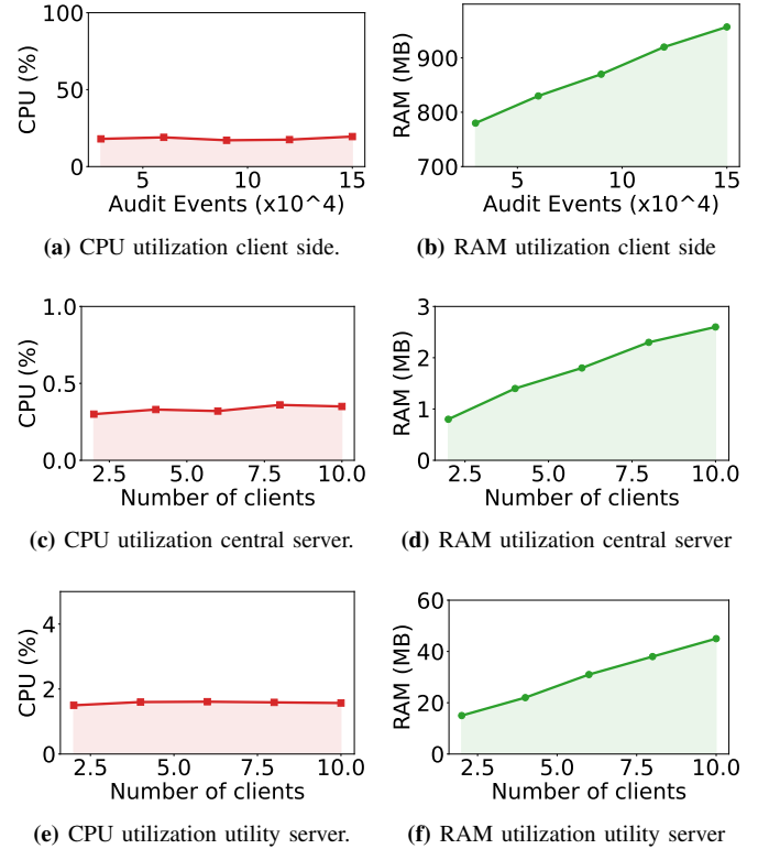
Fig. 3: Resource consumption of various components of MIRAGE.
