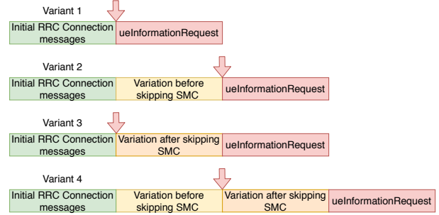
Fig. 4: \beta -undesired-behavior-session variants where \beta =privacy attack on the RLF report. The red arrow points to the location in a benign session where both securityModeCommand and securityModeComplete would have appeared.
