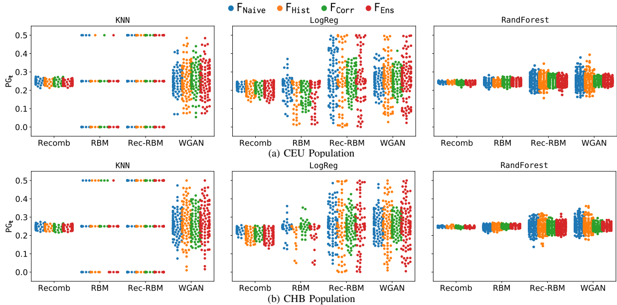
Fig. 5: Privacy Gain (PG) of different models over the two HapMap populations.
