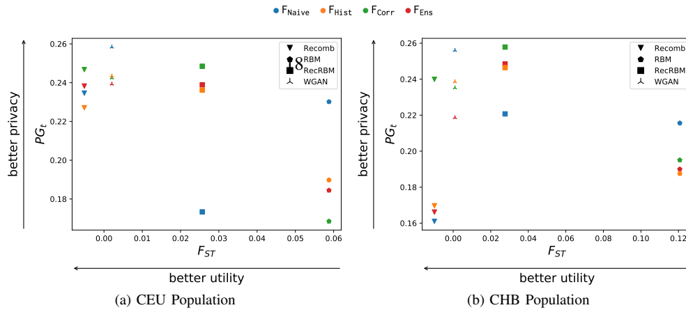
Fig. 16: Fixation index values vs Privacy gain for the HapMap populations.
