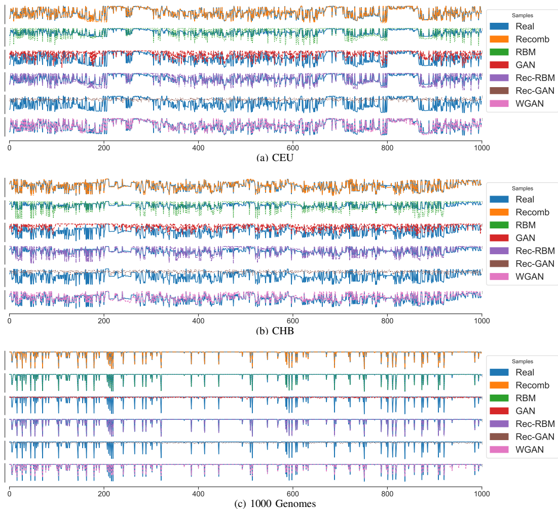
Fig. 1: Major allele frequencies for synthetic data generated by the models, plotted against the real data.
