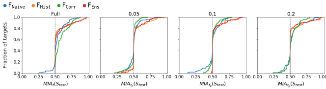
Fig. 9: Accuracy of the Membership Inference Attack with access to full and partial information (0.05, 0.1, and 0.2 ratio) for RBM .
