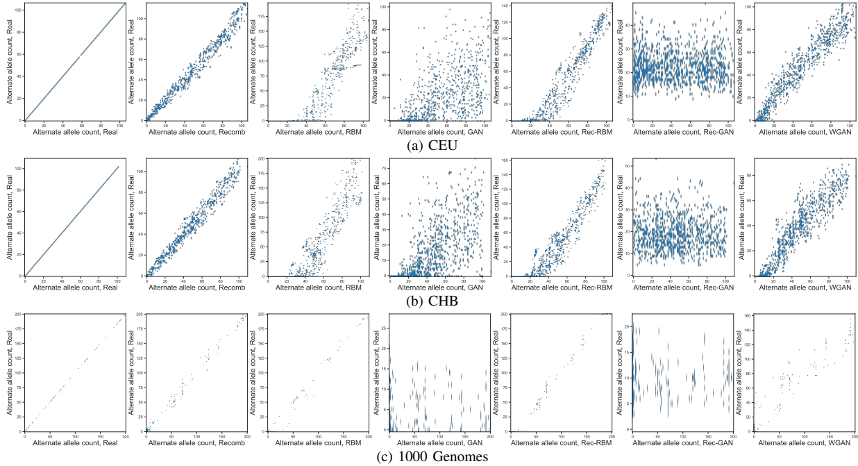
Fig. 12: Alternate allele correlation for the CEU population, the CHB population, and the 1000 Genomes dataset.
