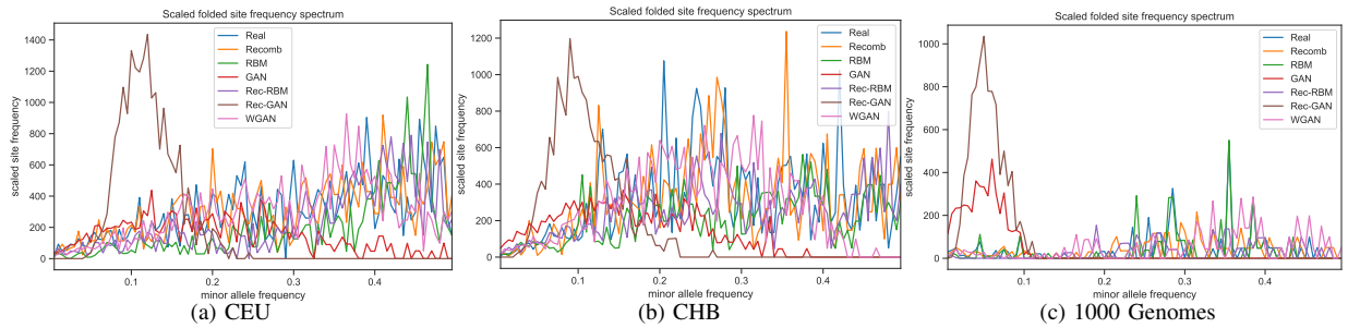
Fig. 13: Frequency spectrum analysis for the CEU population, the CHB population, and the 1000 Genomes dataset.
