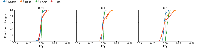
Fig. 8: Privacy Gain (PG) for synthetic samples from Recomb .
