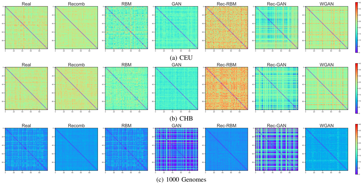
Fig. 14: Pairwise Euclidean Genetic Distance (EGD) between individuals.
