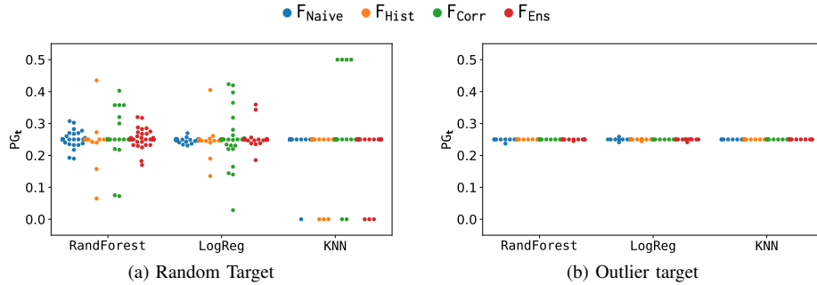
Fig. 6: Privacy Gain (PG) of RBM over the 1000 Genomes dataset.
