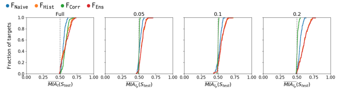
Fig. 7: Accuracy of the Membership Inference Attack with access to full and partial information (0.05, 0.1, and 0.2 ratio) for Recomb .
