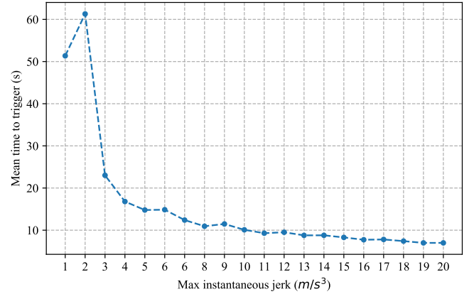
Figure 6: A plot showing the mean time to trigger for various j values for a UAV that uses an IM-20689 inertial sensor. An attacker will be detected in less than 10s if the UAV’s rate of change of acceleration is atleast 10\text{ m/s}^3 .
