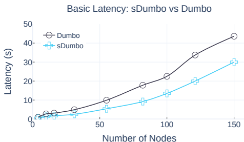
Fig. 9: Basic latency of sDumbo and Dumbo
