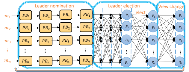
Fig. 3: The structure of AMS19 MVBA [4].
