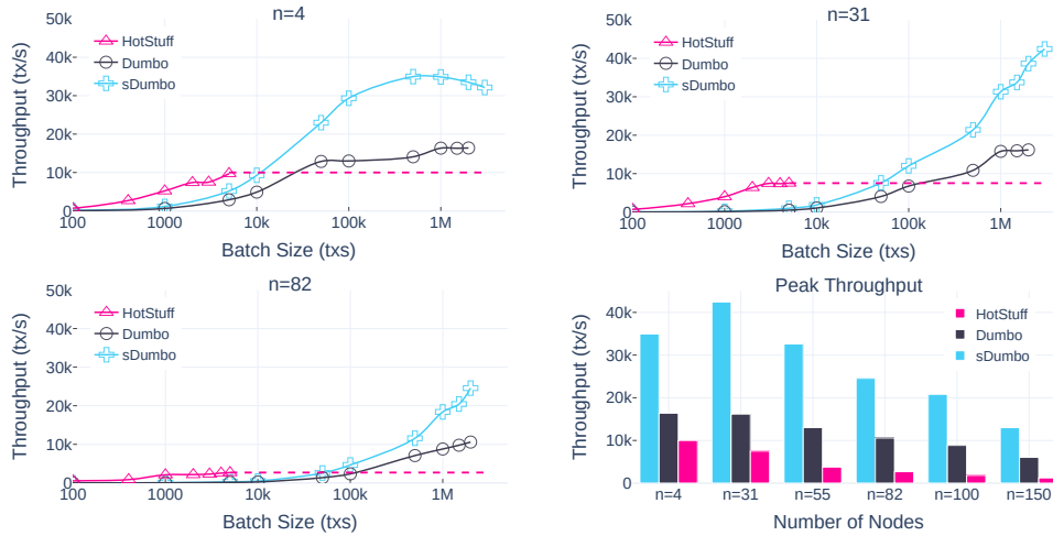
Fig. 8: Throughput of several BFT protocols
