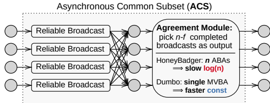
Fig. 1: The execution flow of ACS in HoneyBadgerBFT and Dumbo.
