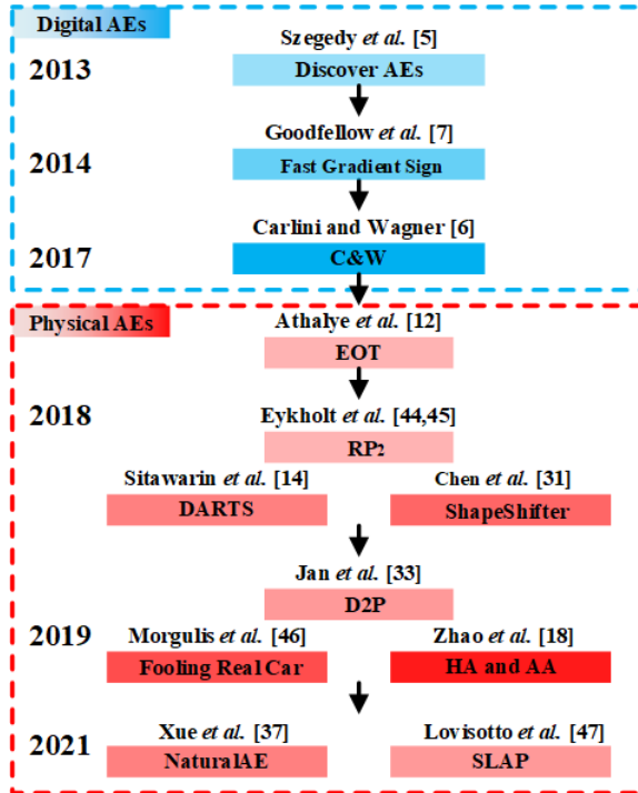
Fig. 10. Adversarial Attacks.
