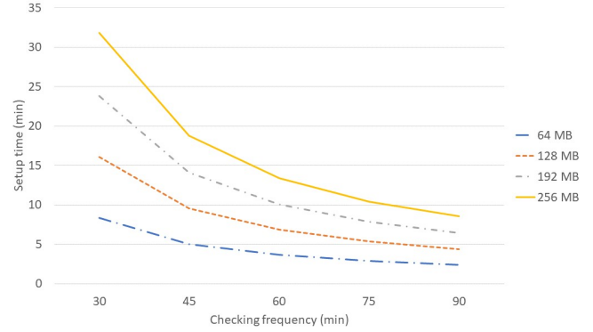
Fig. 5: The compact PoSt setup times for various file sizes and different checking frequency, with \delta = 0.0001 and 30 days data available period.
