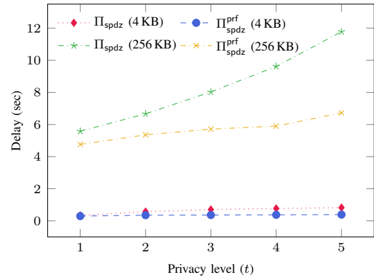
Fig. 15: End-to-end delay with varied privacy levels.
