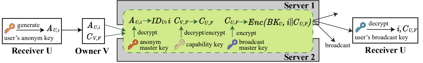
Fig. 8. Sending and receiving a file's capability in Metal-SHARE.
