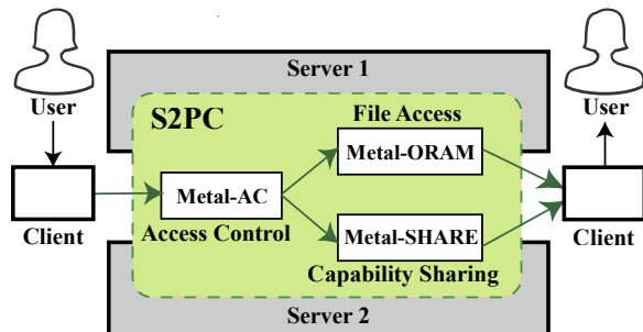
Fig. 2. Metal’s system architecture (described in §II-A).
