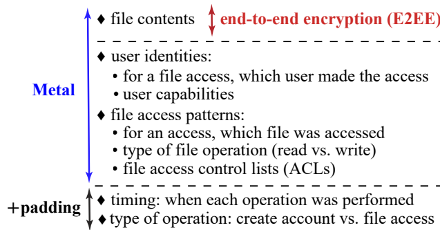
Fig. 1. Scope of data/metadata protected by end-to-end encryption (E2EE) systems and Metal; padding in time and computation hides more metadata.
