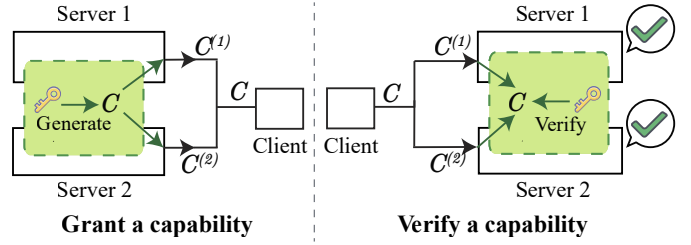
Fig. 4. Metal-AC grants or verifies a capability C using the capability key, which is secret-shared between the two Metal servers.
