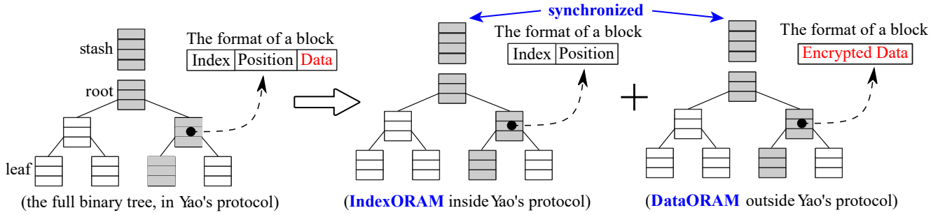
Fig. 5. Metal-ORAM moves data out of Yao's protocol (§V-C). The data is too large to be processed efficiently in Yao's protocol.
