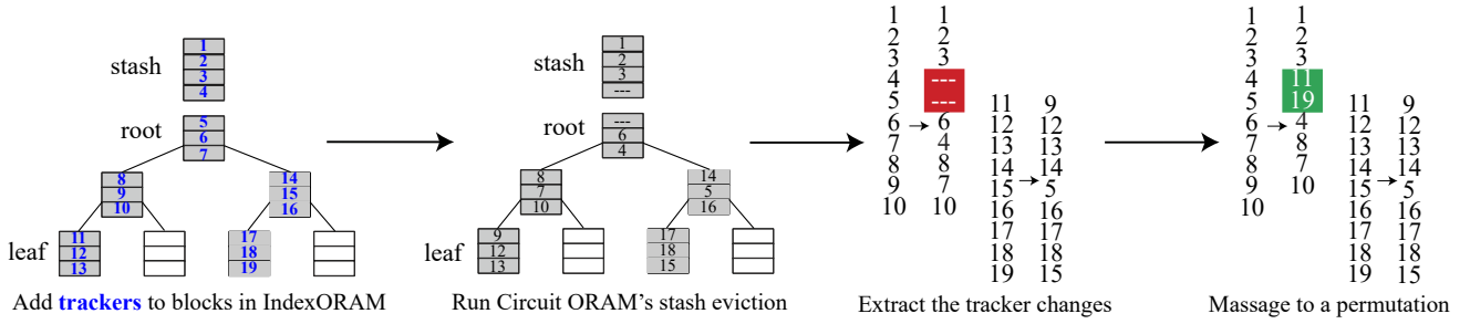
Fig. 6. Metal’s tracking and permutation generation (§V-F).
