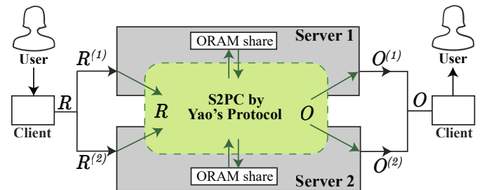
Fig. 3. Metal’s two servers run Yao’s protocol to take user input and access ORAM storage.
