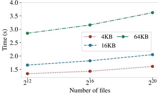
Fig. 10. File access latency vs. the number of files / file size. The result is the average of one hundred measurements.
