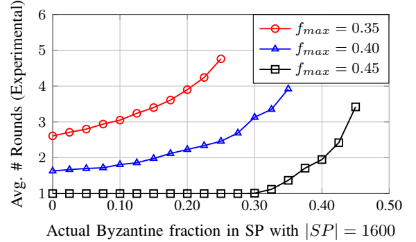
Figure 1: Number of rounds MiRACLE takes to terminate with f \leq f_{max} when designed for worst case ( f = f_{max} ) expected number of rounds for termination to be 5 i.e. R(f_{max}) = 5 . For the case f_{max} = 0.45 , for all f \leq 0.30 , MiRACLE terminates in one round.
