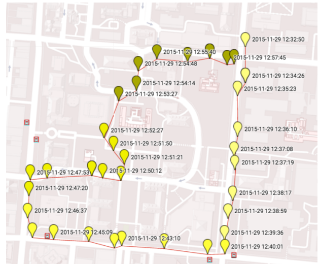
Fig. 9: Inferred trajectory
