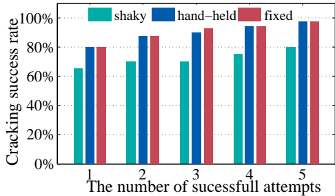
Figure 21. Impact of camera shake. Our approach has the same success rate under the hand-held and the fixed modes and the performance degradation under the shaky mode is modest.
