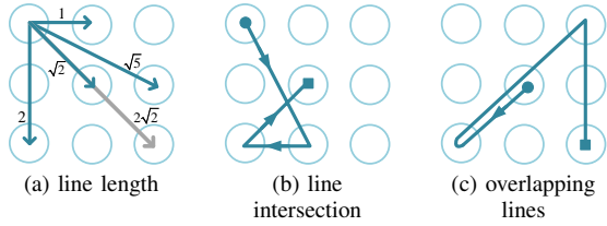
Figure 12. Illustrations of the terminologies used in Equation 2.
