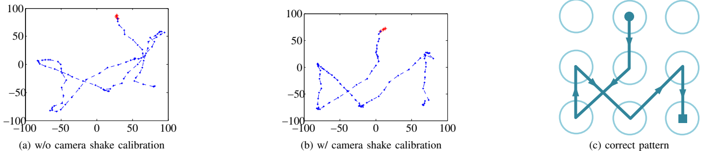
Figure 6. The resulting fingertip movement trajectories without (a) and with (b) camera-shake calibration. The correct pattern is shown in (c). To aid clarity we have transformed (a) and (b) to the user’s perspective.
