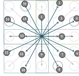
Figure 10. All possible line directions for a 3 \times 3 Android pattern grid.
