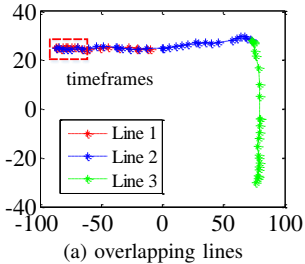
Figure 9. Separating two overlapping line segments by checking the number of overlapping points within a timeframe.
