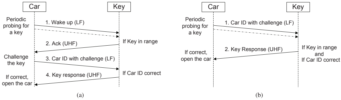
Figure 1. Examples of Passive Keyless Entry and Start system protocol realizations. a) In a typical realization, the car periodically probes the channel for the presence of the key with short beacons. If the key is in range, a challenge-response protocol between the car and key follows to grant or deny access. This is energy efficient given that key detection relies on very short beacons. b) In a second realization, the car periodically probes the channel directly with larger challenge beacons that contain the car identifier. If the key is in range, it directly responds to the challenge.
