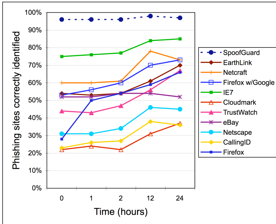
Figure 13: Catch rate of each tool over time using APWG URLs. Note that SpoofGuard's catch rate is estimated after time 0.
