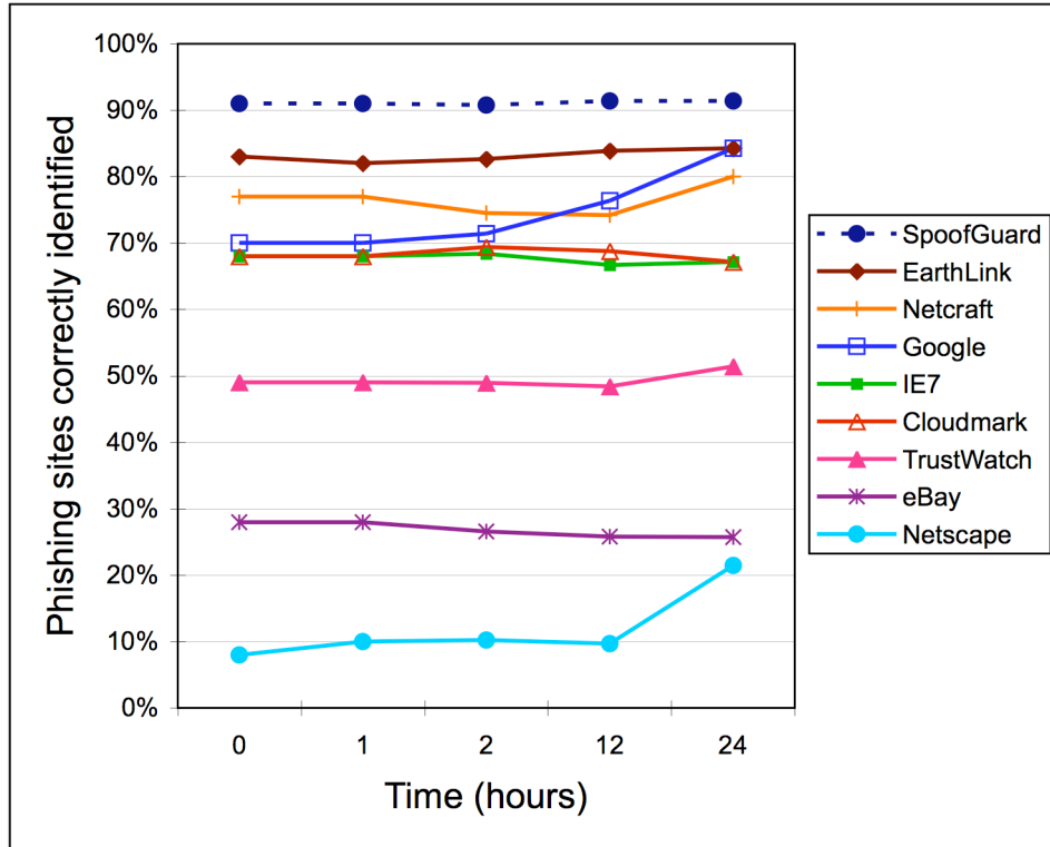
Figure 12: Catch rate of each tool over time using phishtank.com URLs. Note that SpoofGuard's catch rate is estimated after time 0.
