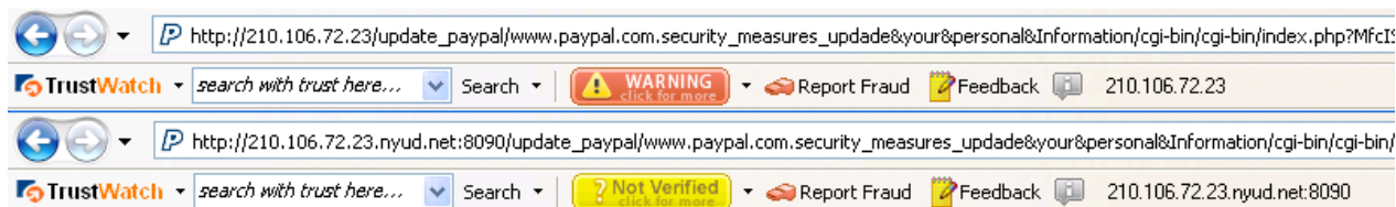
Figure 14: Demonstration of the CDN attack on the TrustWatch tool. The top screenshot shows TrustWatch correctly labeling a site as a phishing scam. The bottom screenshot shows how redirecting that same scam through the Coral CDN causes the same site to be labeled incorrectly.
