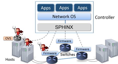
Fig. 3: SPHINX architecture.
