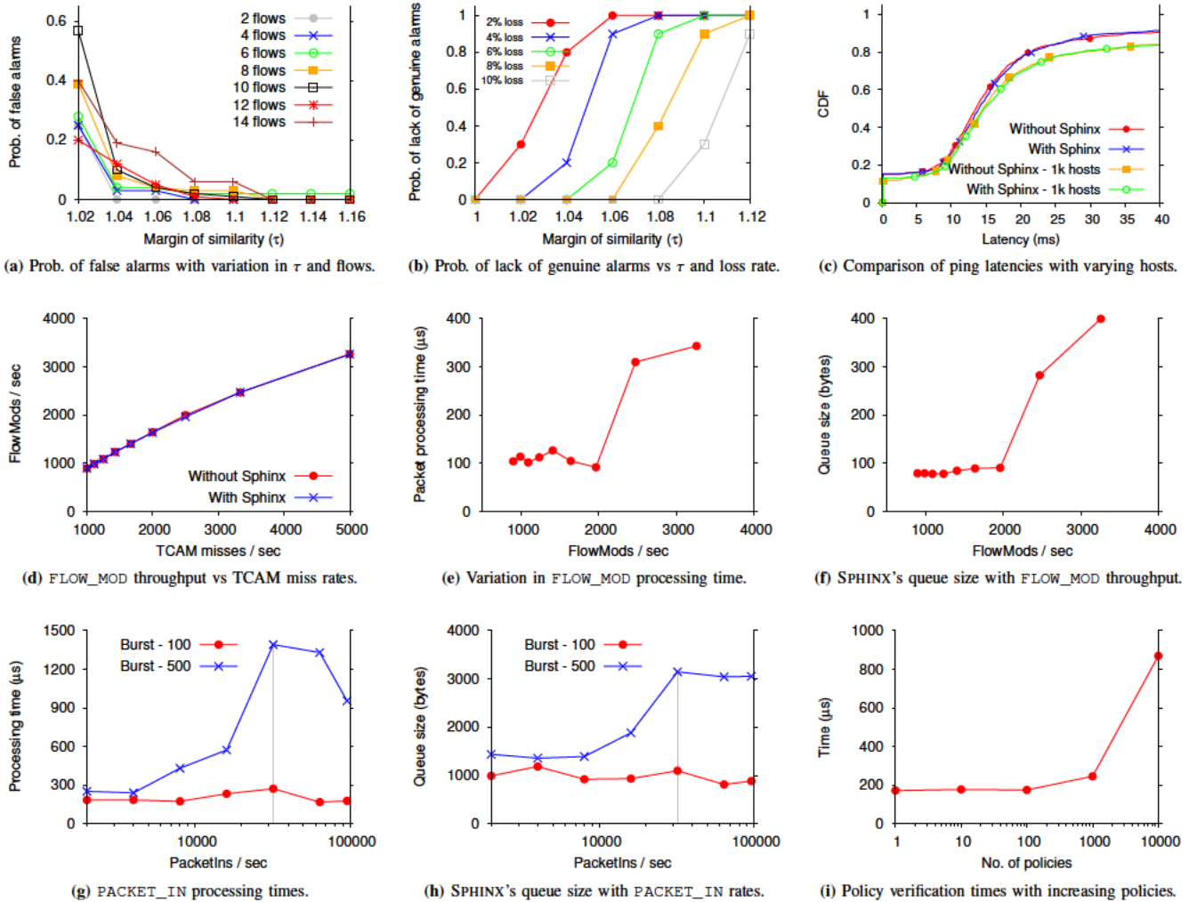
Fig. 10: SPHINX evaluation.
