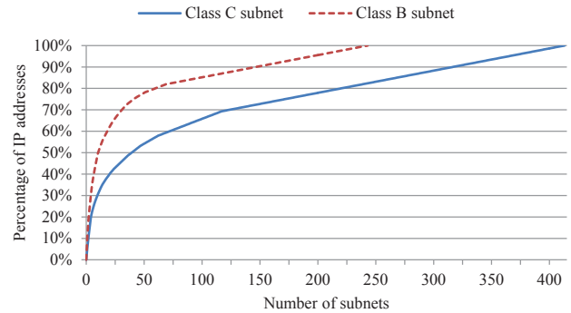
Fig. 5. Cumulative distribution of IP addresses over number of subnets. The total number of class C subnets is 413 and class B subnet is 243. Half of IP addresses observed belong to 40 class C subnets or 10 class B subnets.
