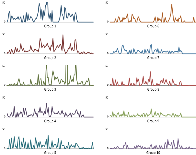
Fig. 12. Emails Per Day - Top 10 Groups. A subset of the top 10 groups show aligned peaks and lulls. Activities tapered off towards the end, partly due the lack of new posts and expiration of existing posts.
