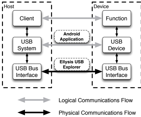
Fig. 3: USB communications model. We observed physical communications via an Ellysis USB Explorer to confirm the correctness of an Android-based protocol analyzer.
