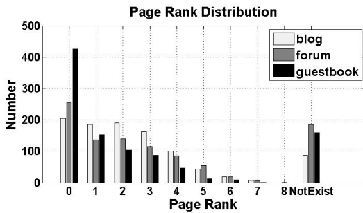
Figure 2. PageRank Score Distribution of Harbors
