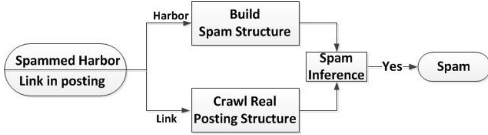
Figure 8. System Architecture of NEIGHBORWATCHER
