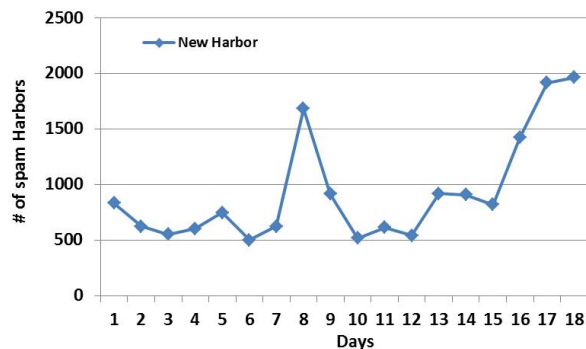
(b) New Spam Harbors
