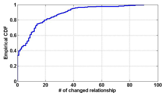
Figure 11. Changed Relationship Distribution
