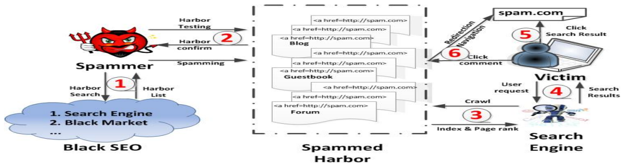
Figure 1. The Workflow of Comment Spamming
