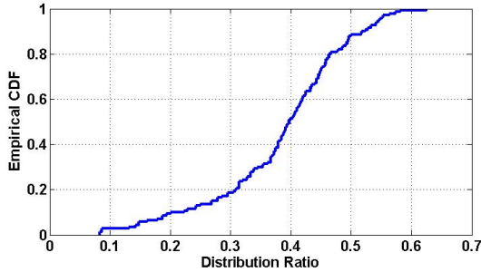
Figure 6. Spam Distribution Ratio
