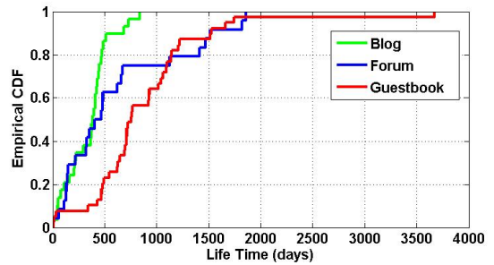
Figure 3. Distribution of Harbor Life Time
