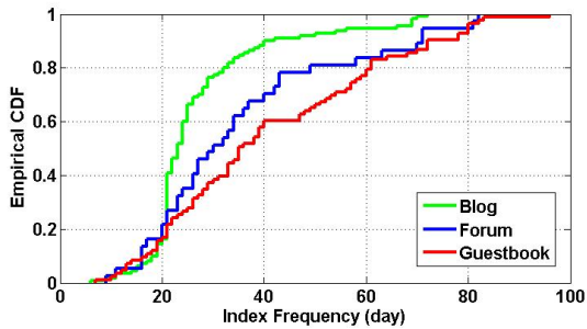
Figure 4. Google Indexing Interval
