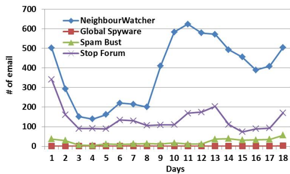
(b) Daily Email
