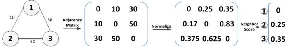
Figure 9. Normalized Neighborhood Relationship Matrix
